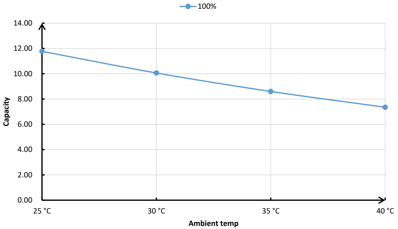
X26-17CP Cooling Capacity Curve
