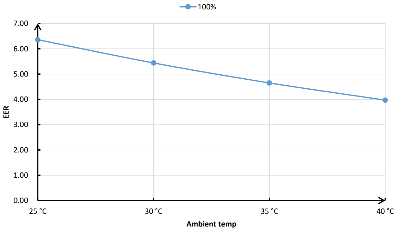
X26-10CP EER Curve
