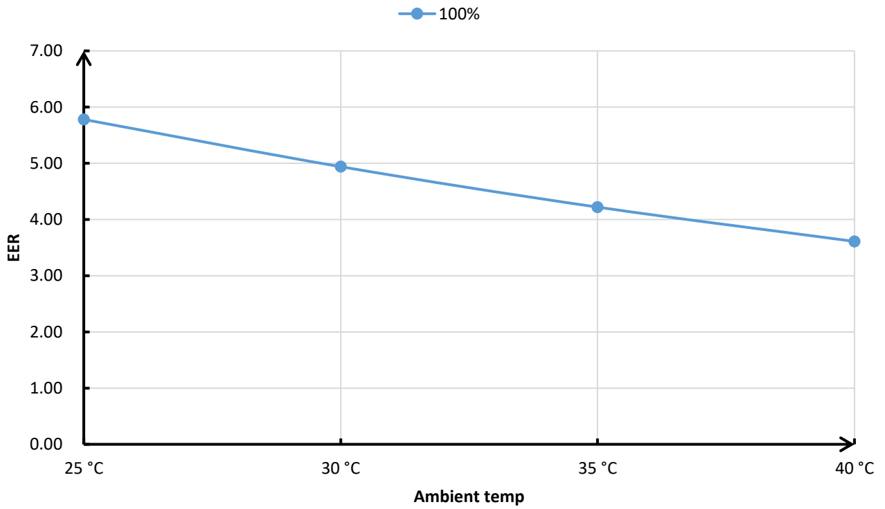
X26-33CPT EER Curve
