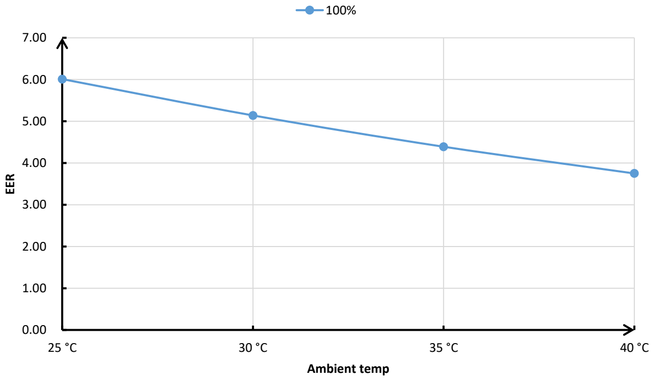
X26-23CP EER Curve
