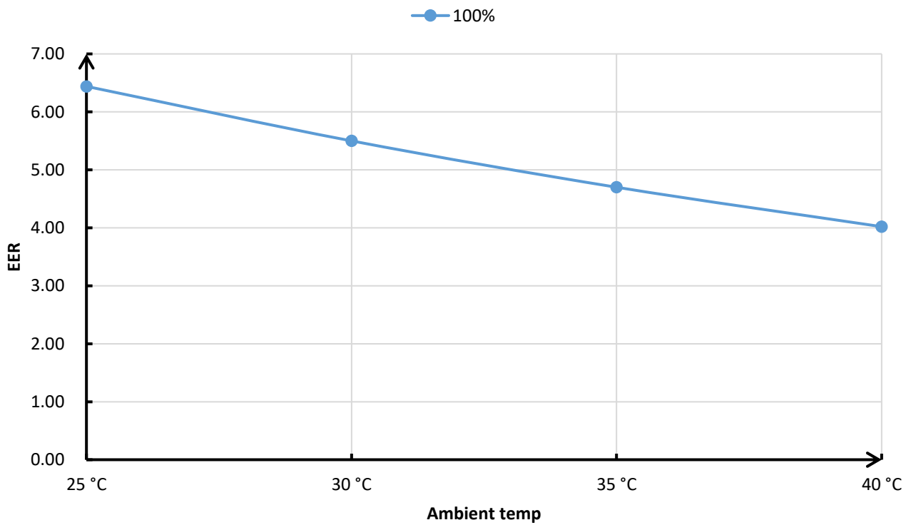
X26-12CP EER Curve
