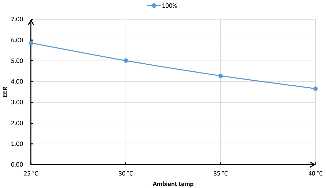
X26-17CP EER Curve
