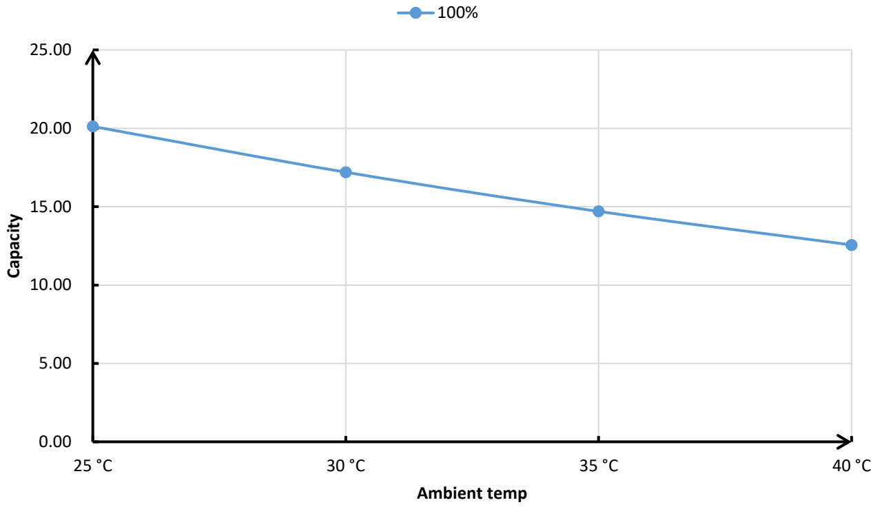
X26-33CPT Cooling Capacity Curve
