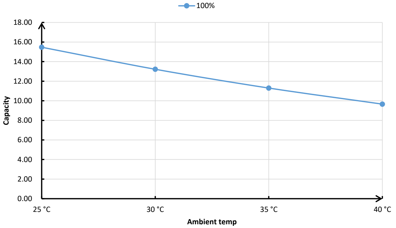
X26-23CP Cooling Capacity Curve
