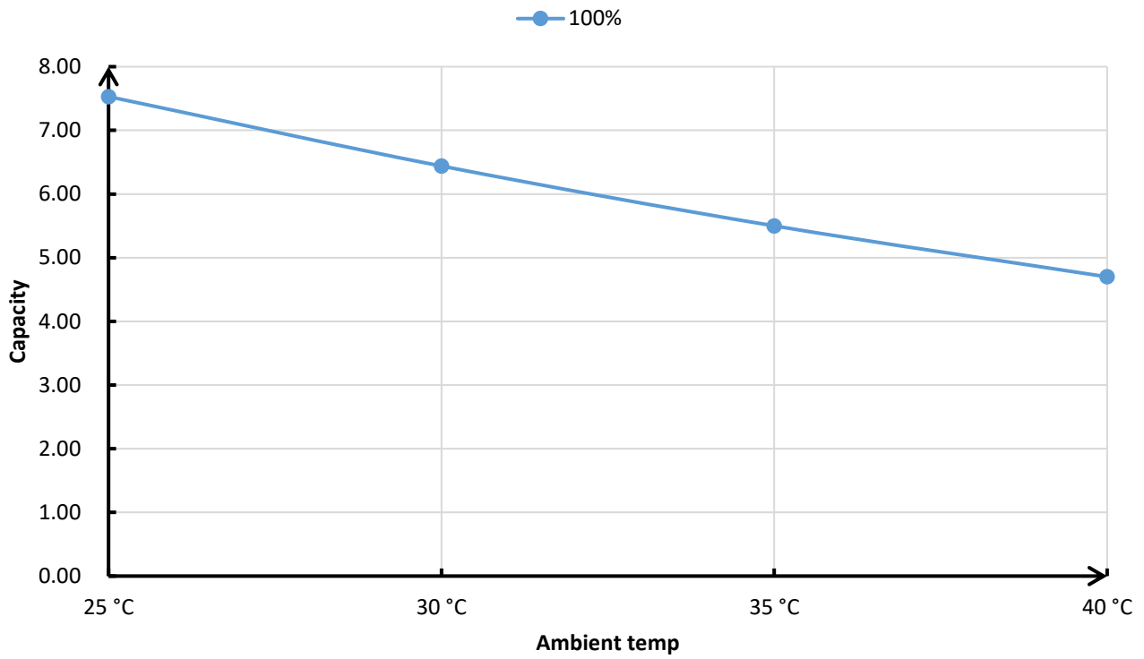
X26-12CP Cooling Capacity Curve
