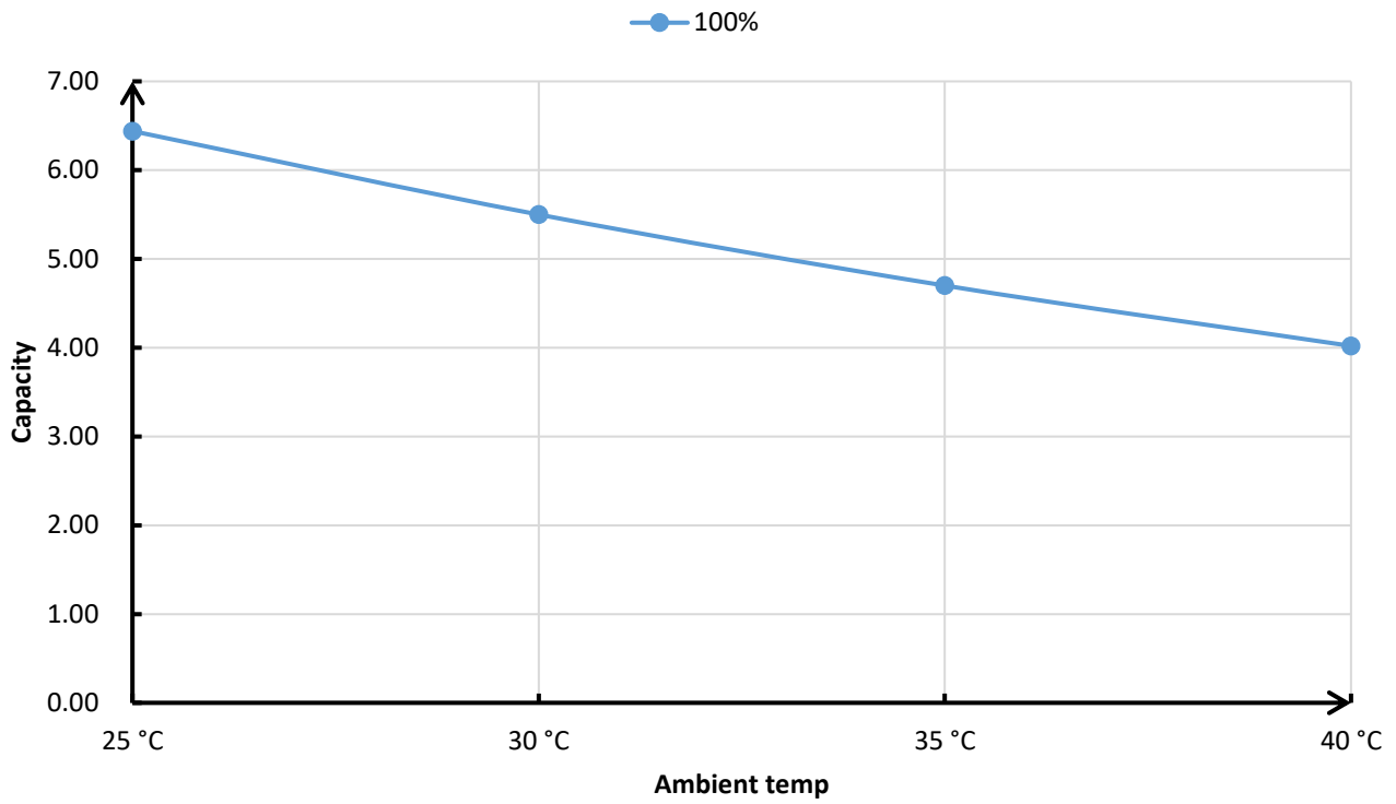
X26-10CP Cooling Capacity Curve
